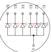
LED CIRCUIT DIAGRAM
